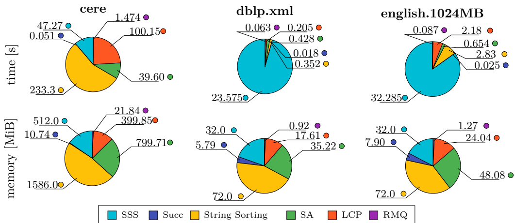
■ Figure 3 Snapshots of construction time and memory usage during construction for different phases of sss_{512} (same as sss_{512}^p ).
